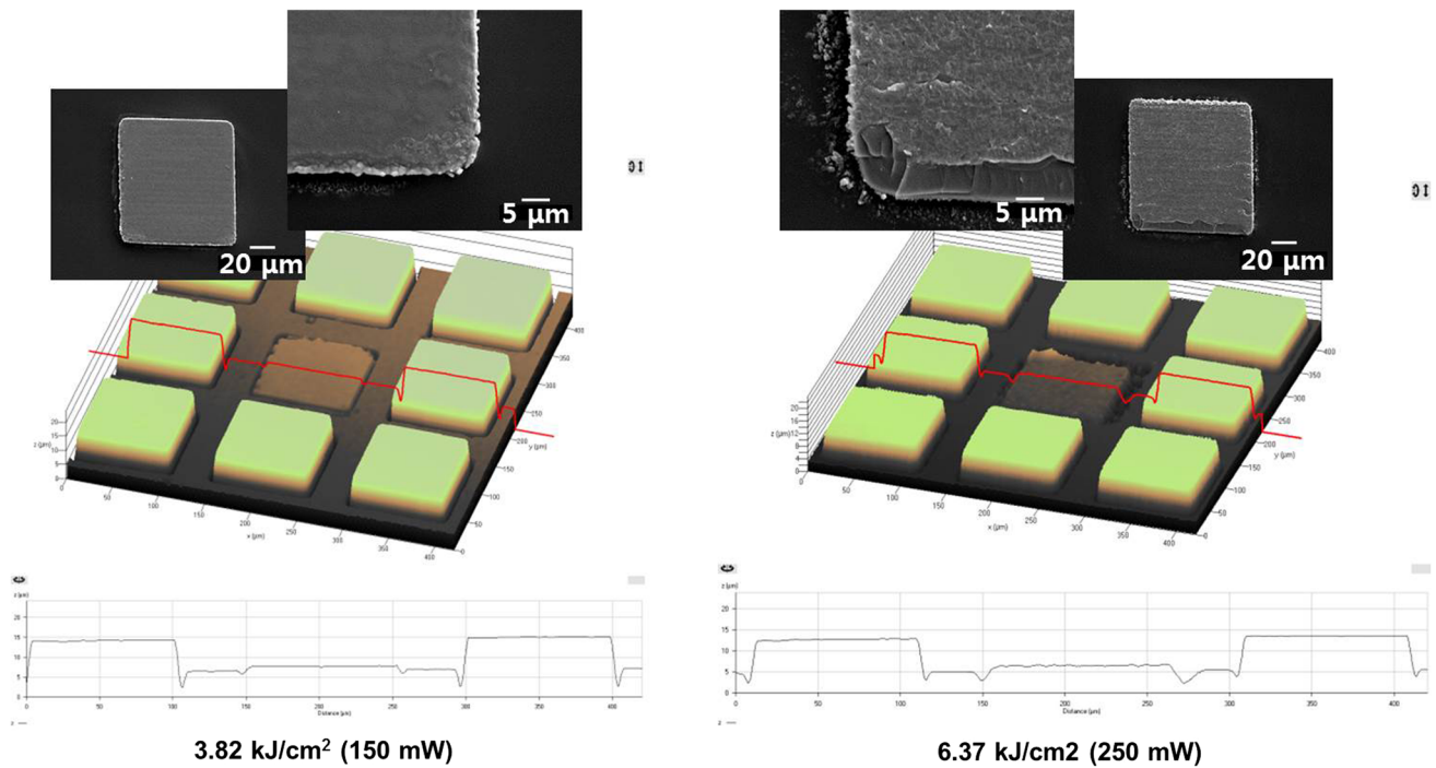
Fig. 4 Images of the GaN surface and profile contour of sapphire the defocused lengths of 450 \mu\text{m} with the fluence of 3.82 \text{ kJ/cm}^2 (150 mW) and 6.37 \text{ kJ/cm}^2 (250 mW)
