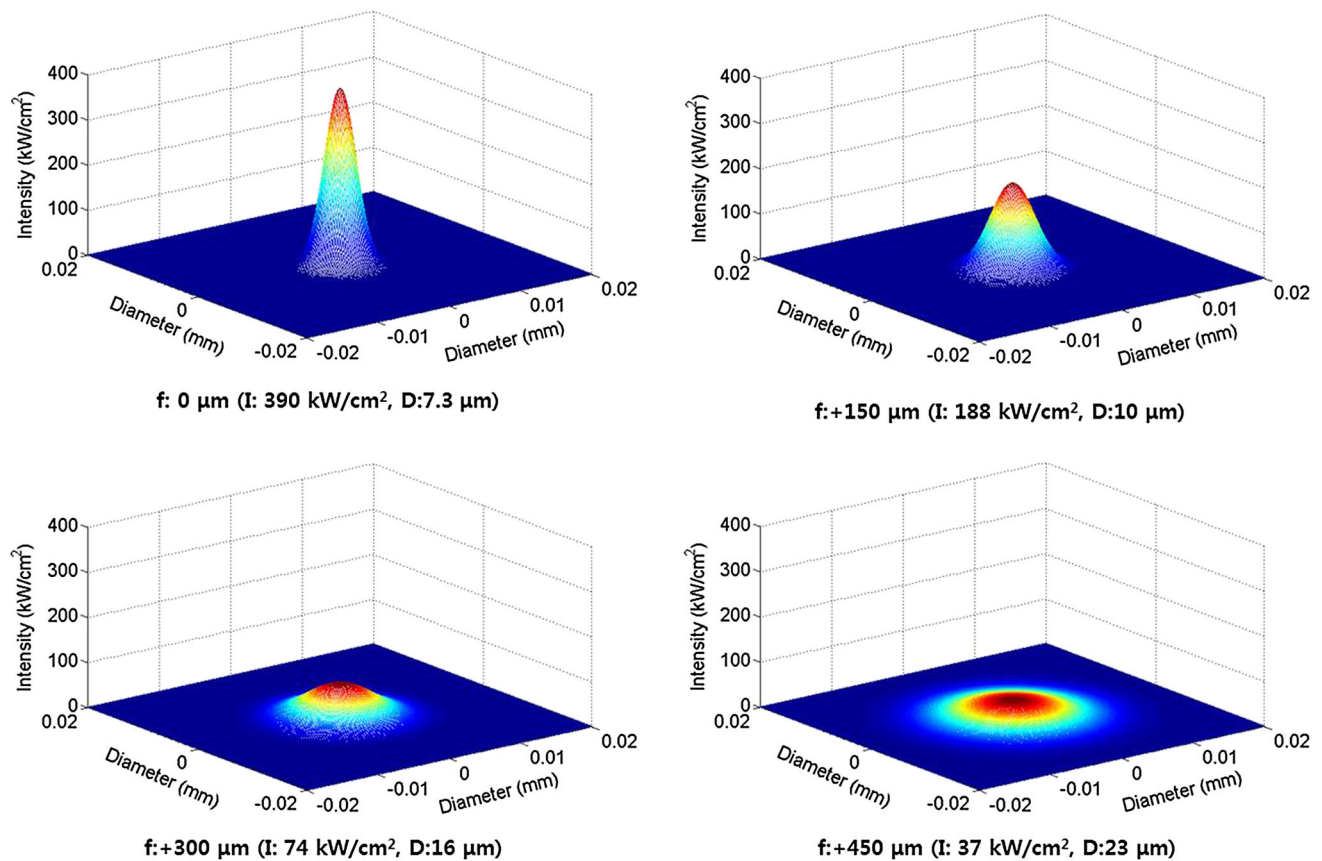
Fig. 5 Intensity distribution changes with respect to the defocused length, with a power of 150 mW and a focal beam size of 7.3 \mu\text{m}
